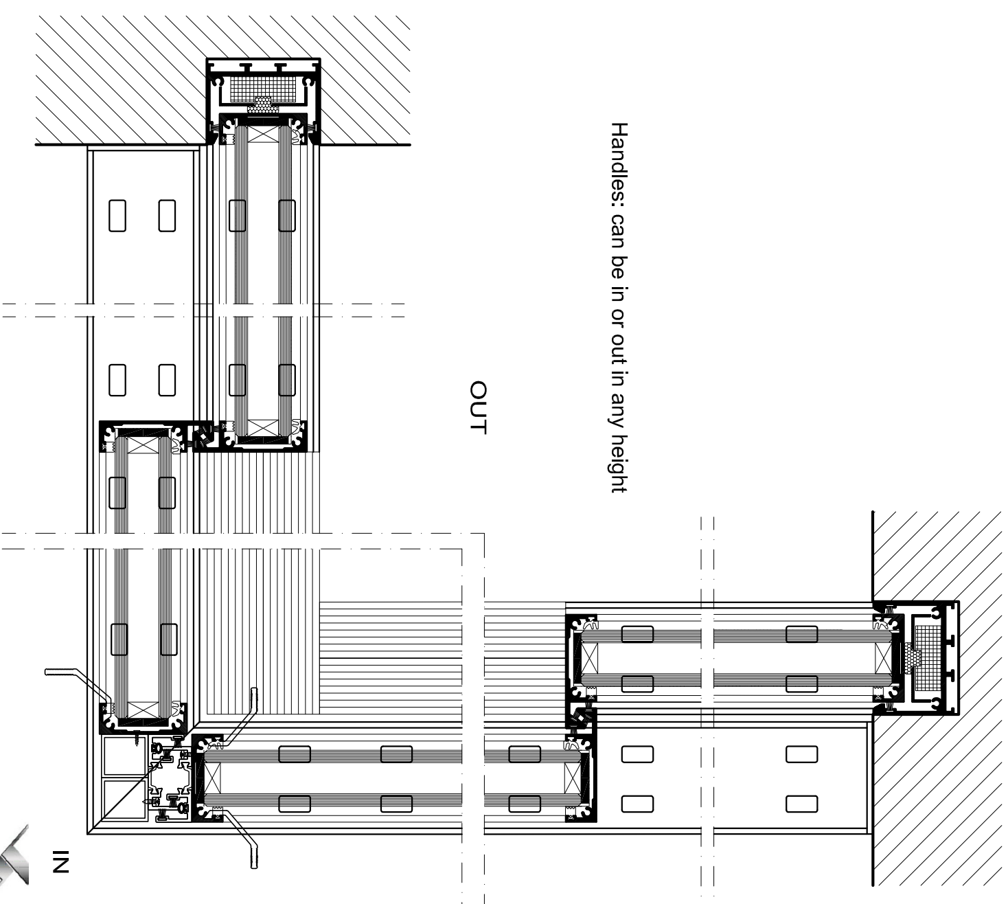
HORIZONTAL SECTION
